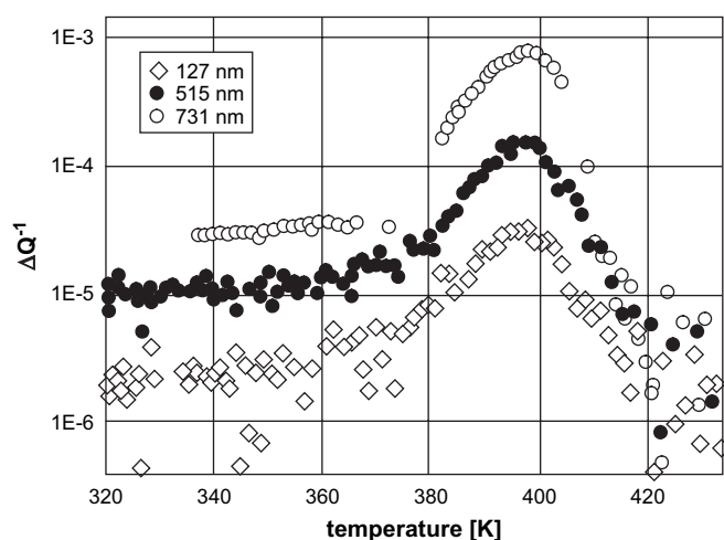
Fig. 3. Mechanical loss spectra containing the \alpha -relaxation, i.e. the glass transition of thick films. The eigenfrequency of the sample is 200 Hz.
