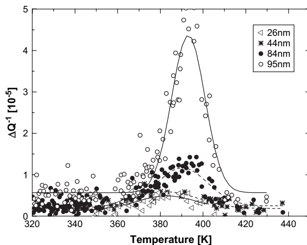
Fig. 4. Mechanical loss spectra of thin films after subtracting the silicon contribution. The eigenfrequency of the sample is 100 Hz.
