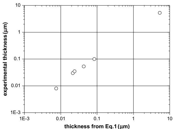
Fig. 2. Thickness of the PS films determined experimentally by SEM from cross-sections of the film/substrate composite and from frequency shifts via Eq. (1).
