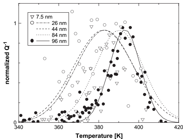
Fig. 5. Data from Fig. 4 but normalized to the same heights and fitted to Gaussian functions. The eigenfrequency of the sample is 100 Hz. The triangles not shown in Fig. 4 correspond to a 7.5 nm thick PS film.
