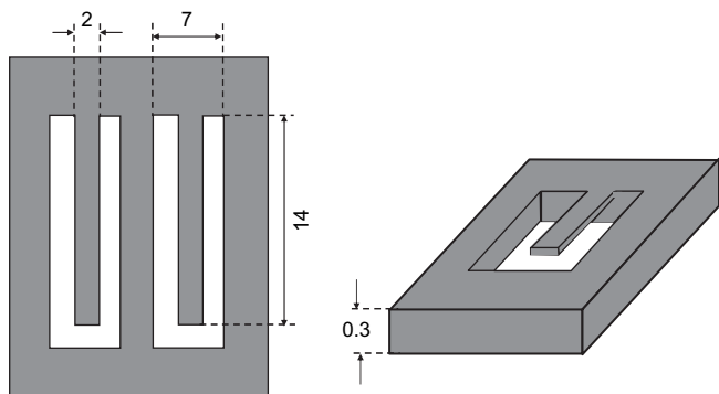
Fig. 1. A top view of the wet etched cantilevers (left). The vibrating reeds in this figure are surrounded by white colour. After etching the piece is broken along the symmetry axis and one of the parts is presented on the right hand side in 3D projection. The numbers presented in the figure are in mm.
