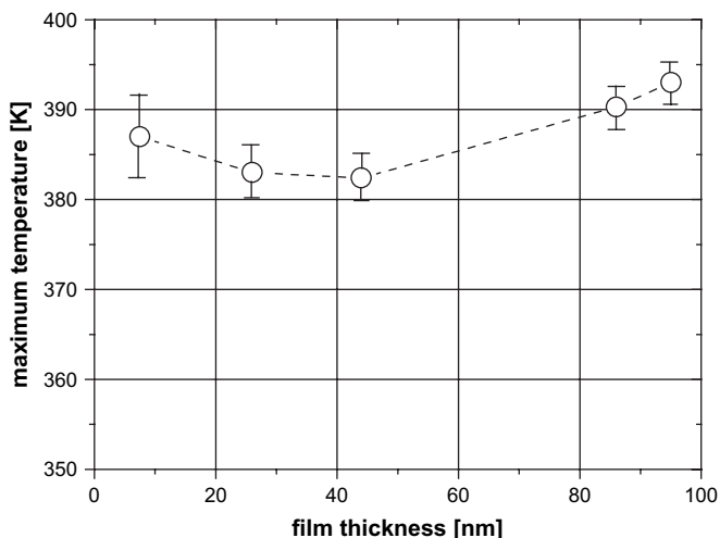
Fig. 6. Peak temperatures T_{max} as a function of film thickness. T_{max} and its error bars are obtained from a least square fit of Gaussian functions to the data between 340 and 420 K. The dashed line is drawn to guide the eyes.
